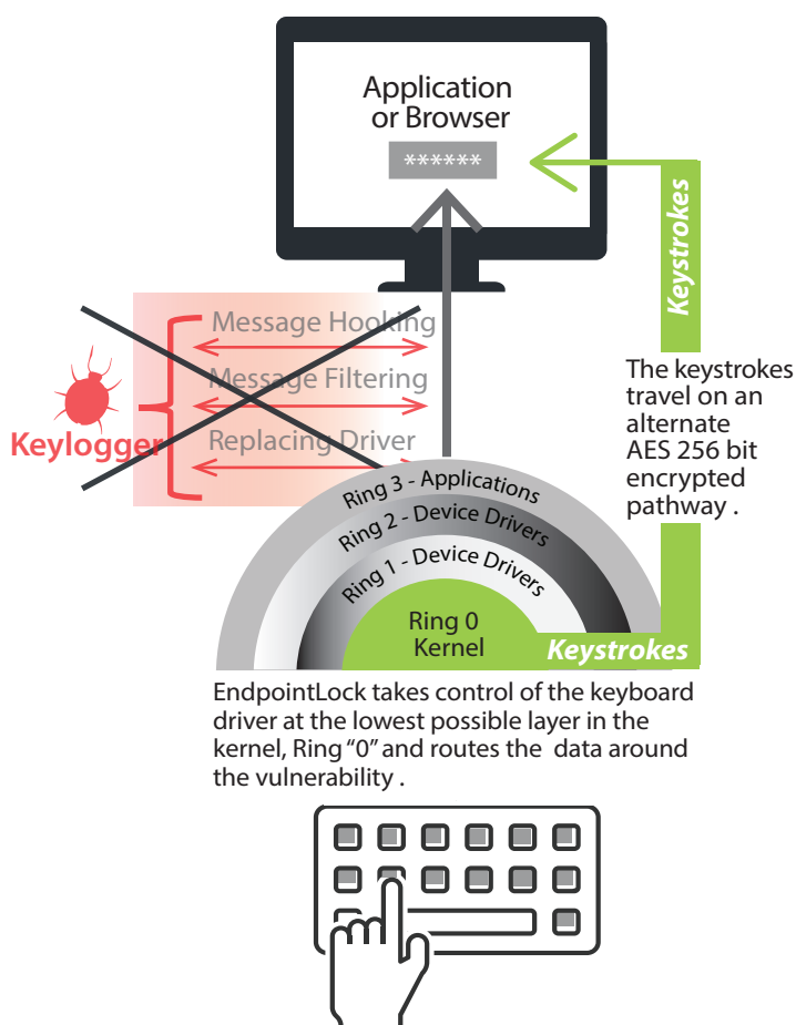
FIGURE 2: KTLS (Keystroke Transport Layers Security)
